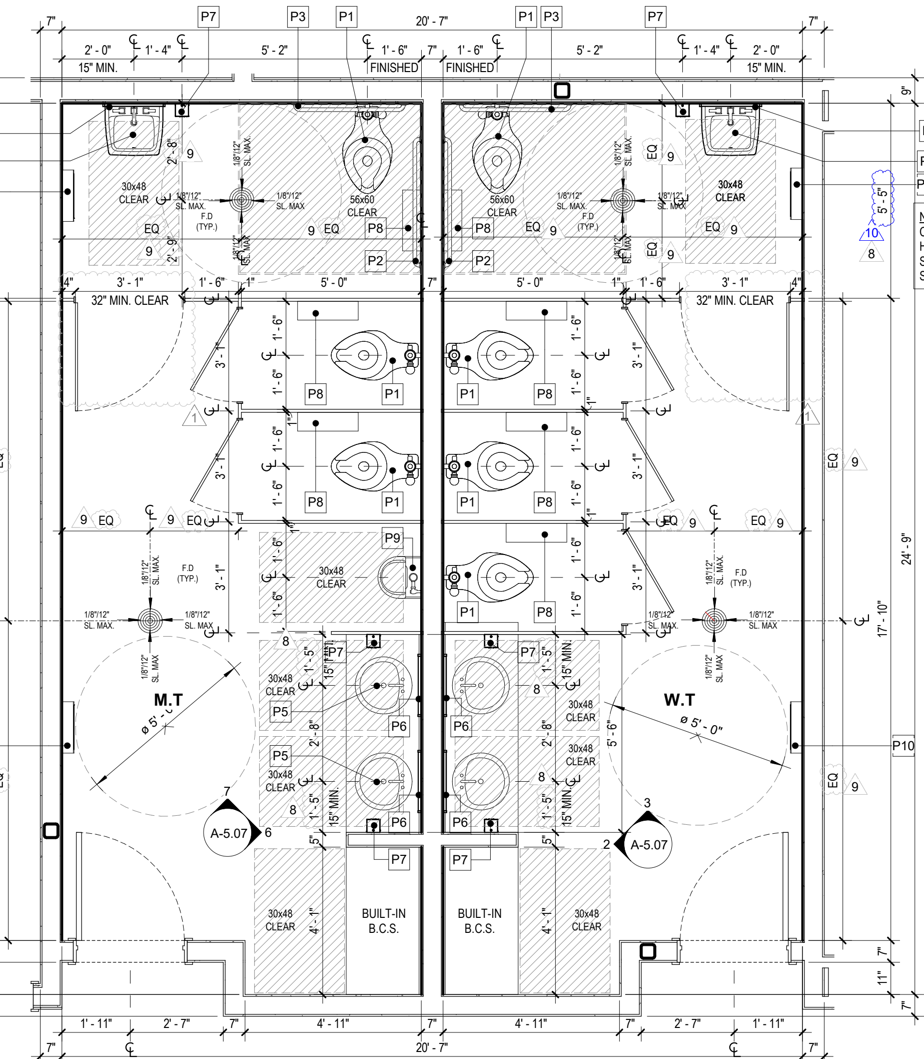
1 COMMUNITY CENTER RESTROOMS
