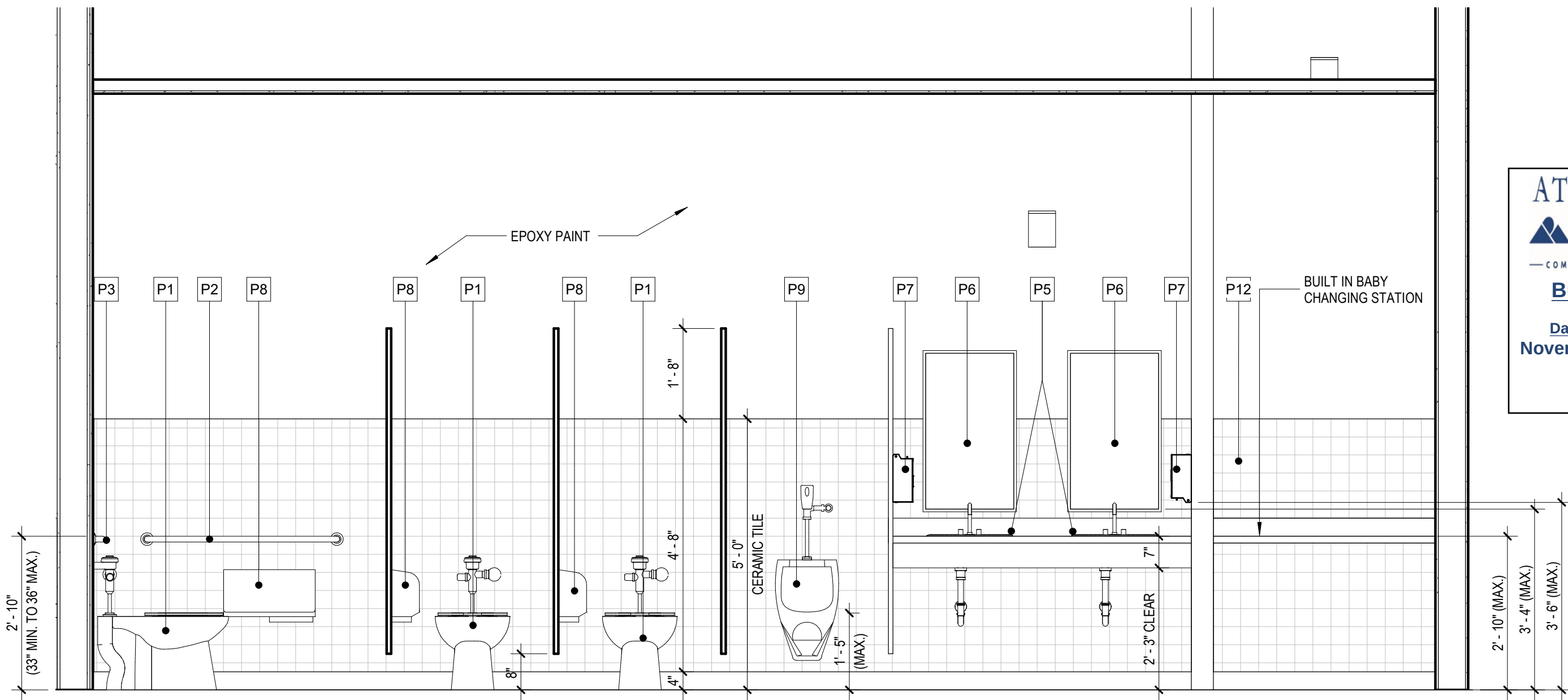
6 MEN RESTROOM ELEVATION
