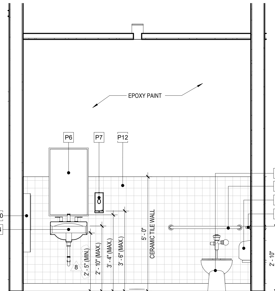
7 MEN RESTROOM ELEVATION
