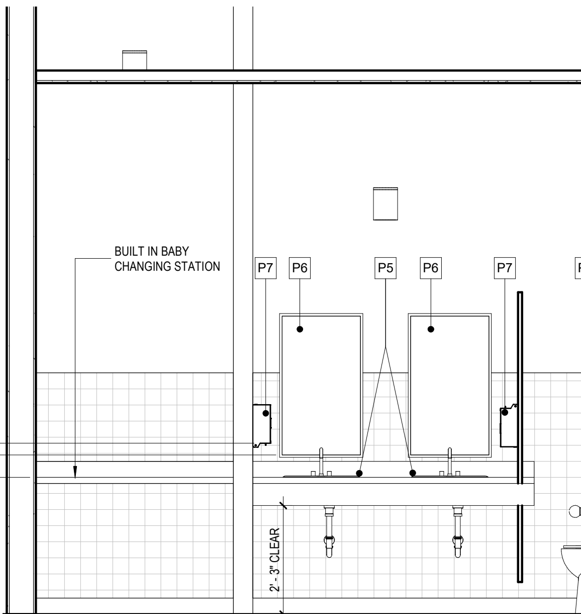
2 WOMEN RESTROOM ELEVATION
